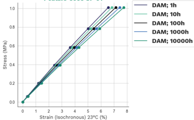
Stress-strain (Isochronous) 23°C Pebax® 3533 SP 01
