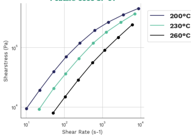
Shearstress-shear rate Pebax® 3533 SP 01
