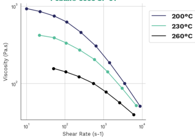
Viscosity-shear rate Pebax® 3533 SP 01
