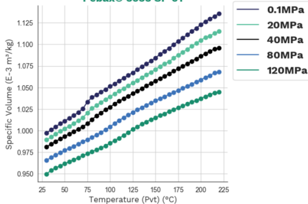
Specific volume-temperature (pvT) Pebax® 3533 SP 01
