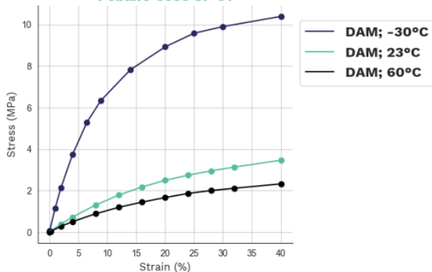
Stress-strain Pebax® 3533 SP 01
